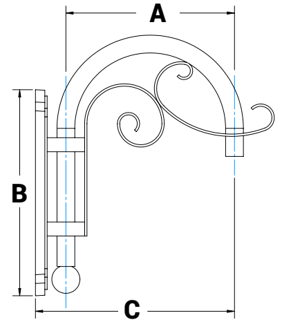
A17 Small Wall Mount
